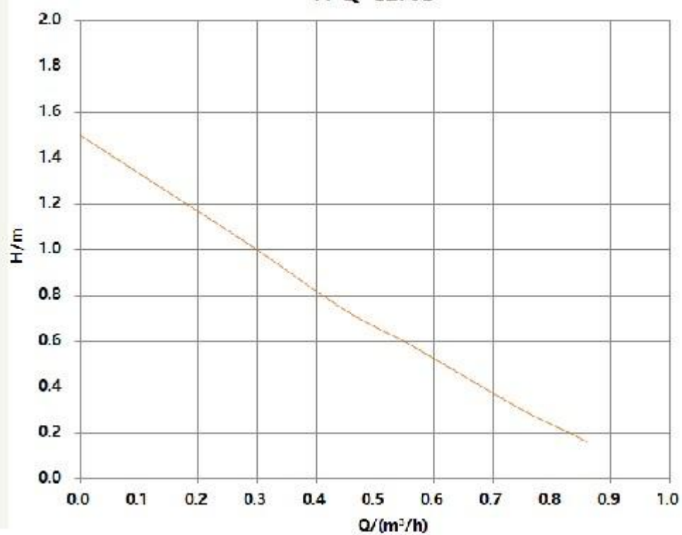
H-Q curve
