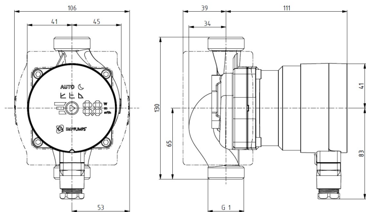
Dimension drawing
