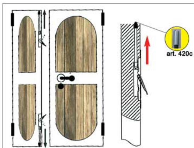
Paletti a leva azione semplice Verrous a levier simple action Single action flush bolt Pasador de embutir simple accion
