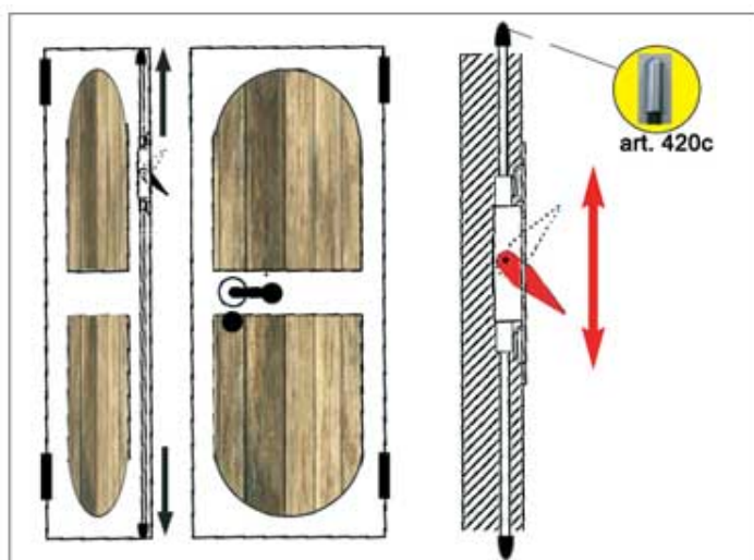
Paletti a leva doppia azione Verrous a levier double action Double acting flush bolt Pasador de embutir doble accion
